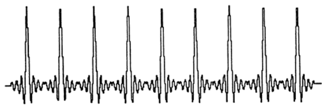
Figure 3-5, \text{Sin}(x)/x Waveform Loaded Into Segment 1
