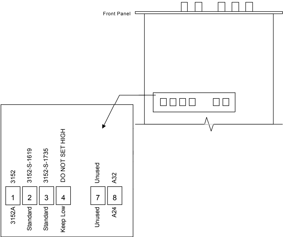
Figure 2-2, 3152 Emulation Mode and Address Space Switch
